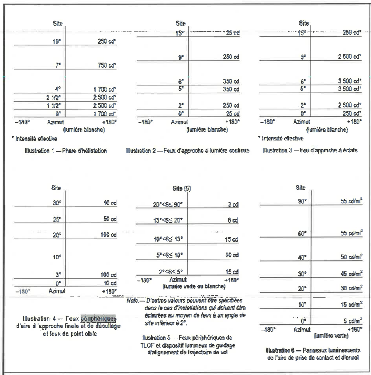
Figure 5-12. Diagrammes isocandelas
